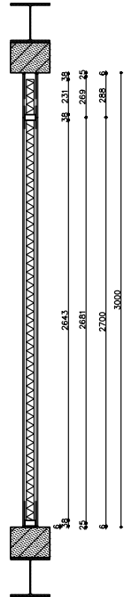
VERTICAL SECTION
