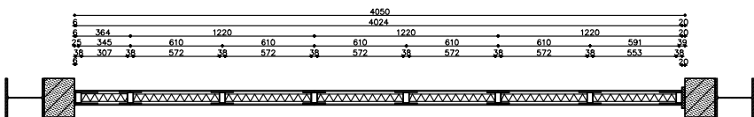
HORIZONTAL SECTION
